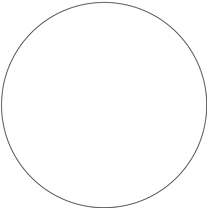
Sketch 3 Capsule Stain
