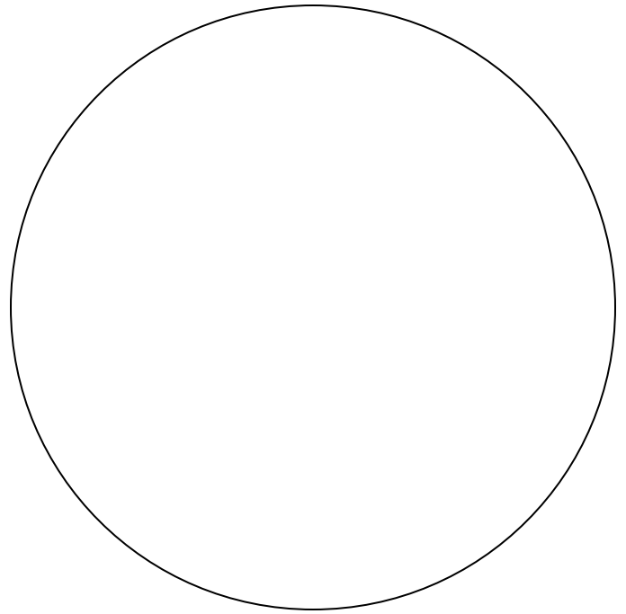
Sketch 6 Gram Stain
