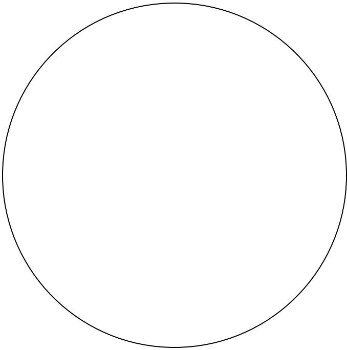
Sketch 1 Simple Stain
