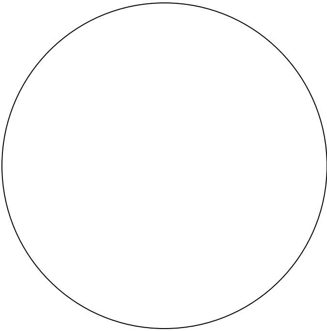
Sketch 5 Negative Stain
